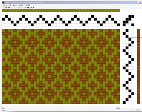
Dobby weaving pattern
